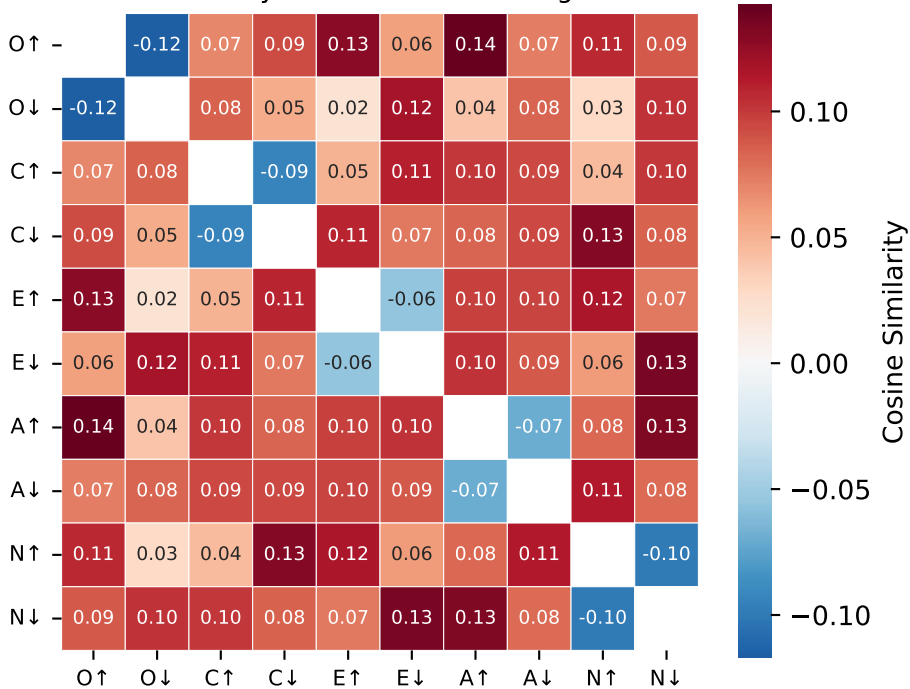
Cosine Similarity of Persona LoRA Weight Vectors
