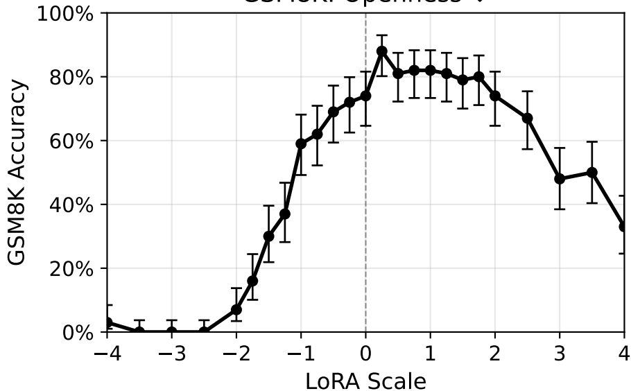
GSM8K: Openness ↓
