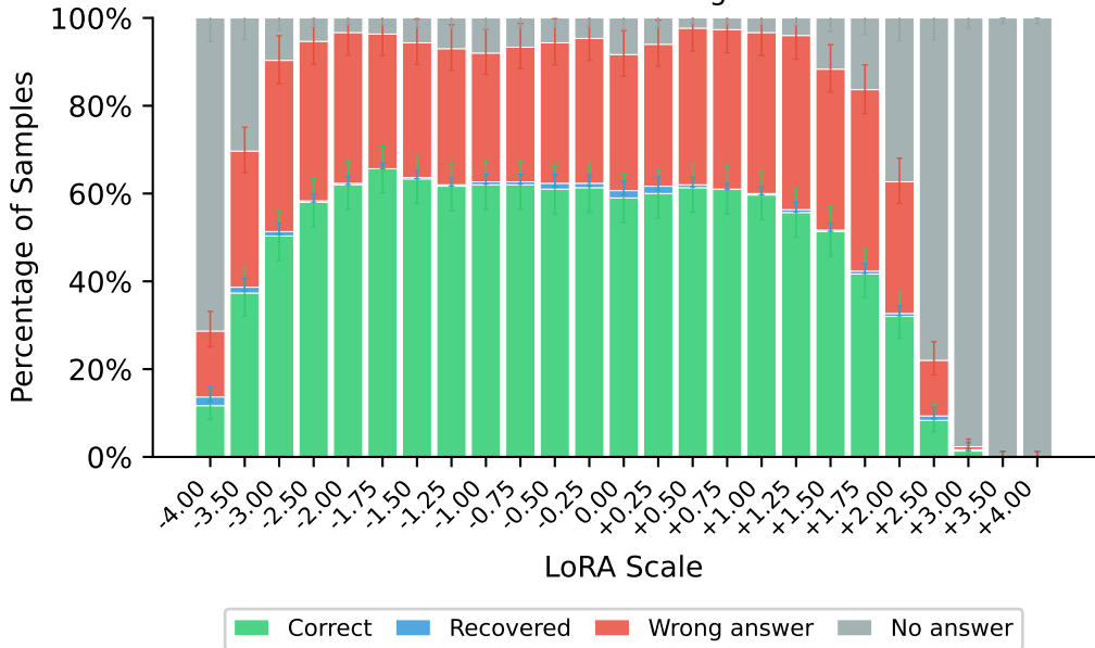
MMLU LoRA Scaling: C ↓
