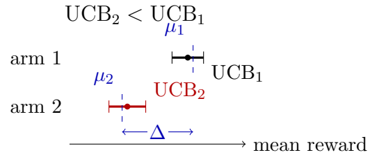
Figure 4.2. Why UCB stops exploring a suboptimal arm. Solid segments are learner-visible confidence intervals, dots are empirical means, and dashed blue markers are the true means. While the intervals overlap, optimism may select arm 2. Once its radius is small relative to the true gap \Delta , its UCB falls below that of the optimal arm. On the clean event, selecting arm 2 requires \Delta \leq 2r_2 .
