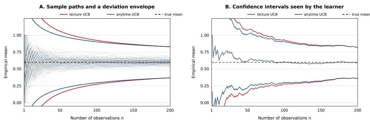
Figure 4.1. Two views of confidence for one Bernoulli arm with \mu = 0.6 and T = 200 . The red lecture UCB radius is r_L(n) = \sqrt{2\log(T)/n} ; the blue anytime UCB radius is r_A(n) = \sqrt{2\log(n)/n} for n \geq 2 . Left: 150 simulated empirical-mean paths and the two deviation envelopes around \mu . Right: one realized path and the corresponding learner-visible intervals. The anytime radius is tighter before the horizon and meets the lecture radius at n = T . The figure uses a fixed random seed.
