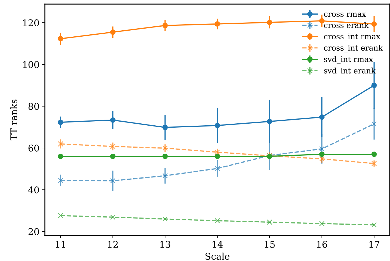
Scale vs rmax & erank
