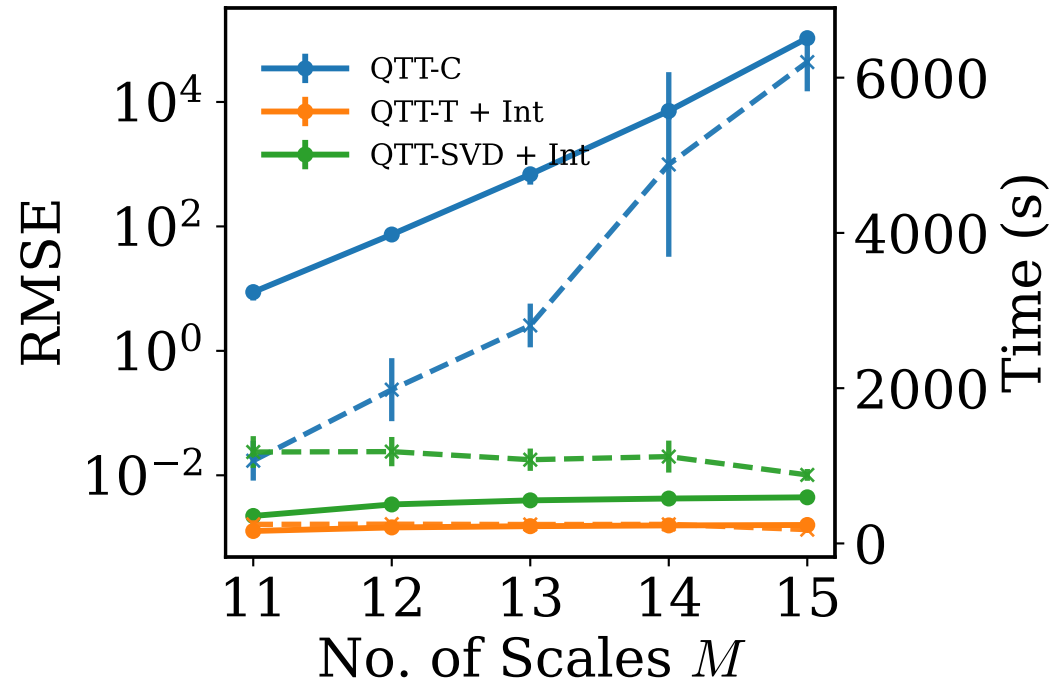
a. Mean error and Time
