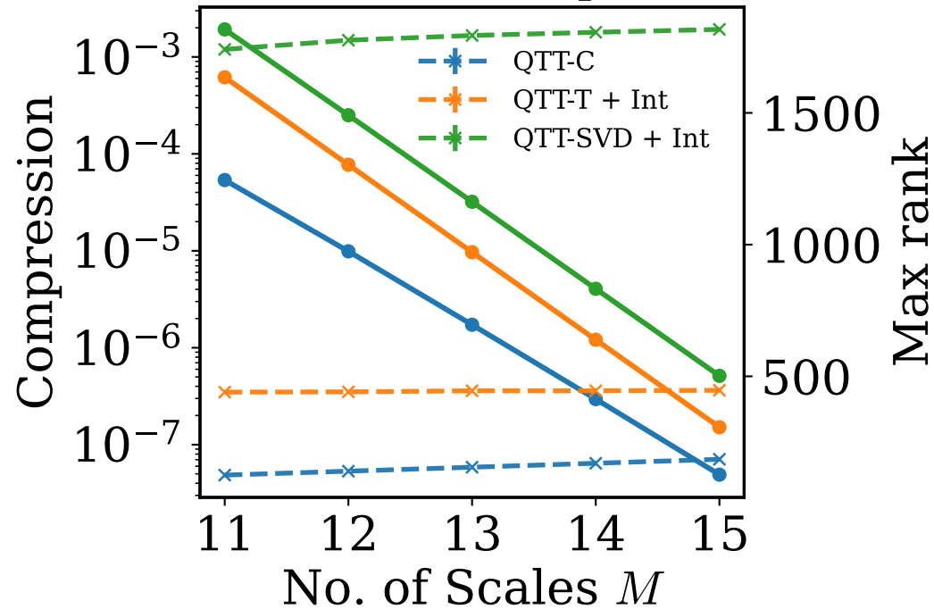
b. Rank and Compression
