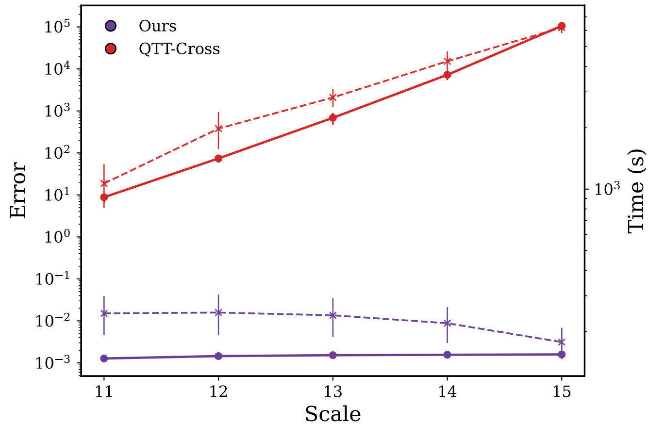
Scale vs Error & Time
