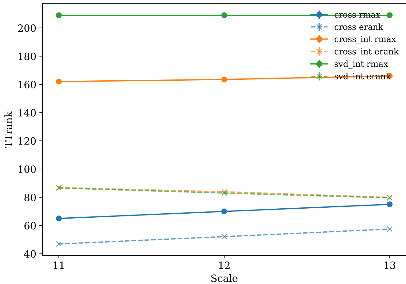
Scale vs rmax &amp; erank
