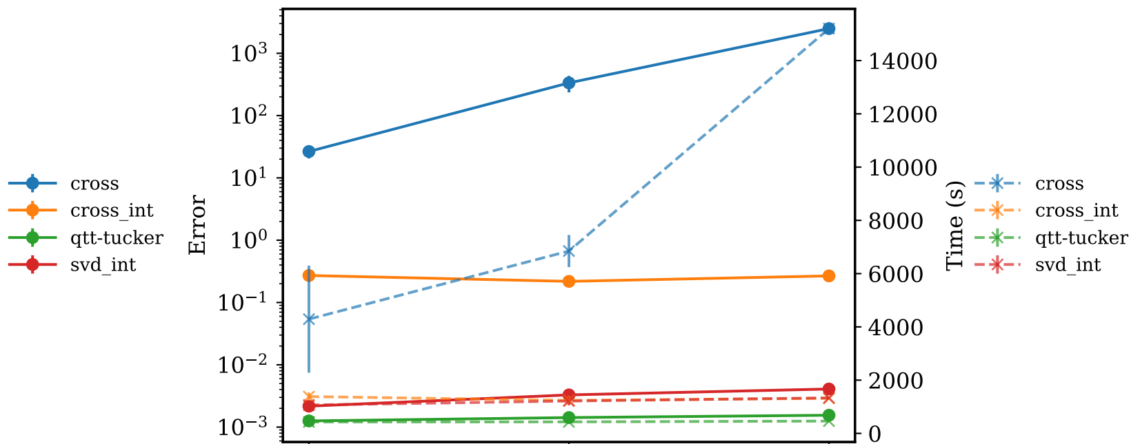
Scale vs Error & Time
