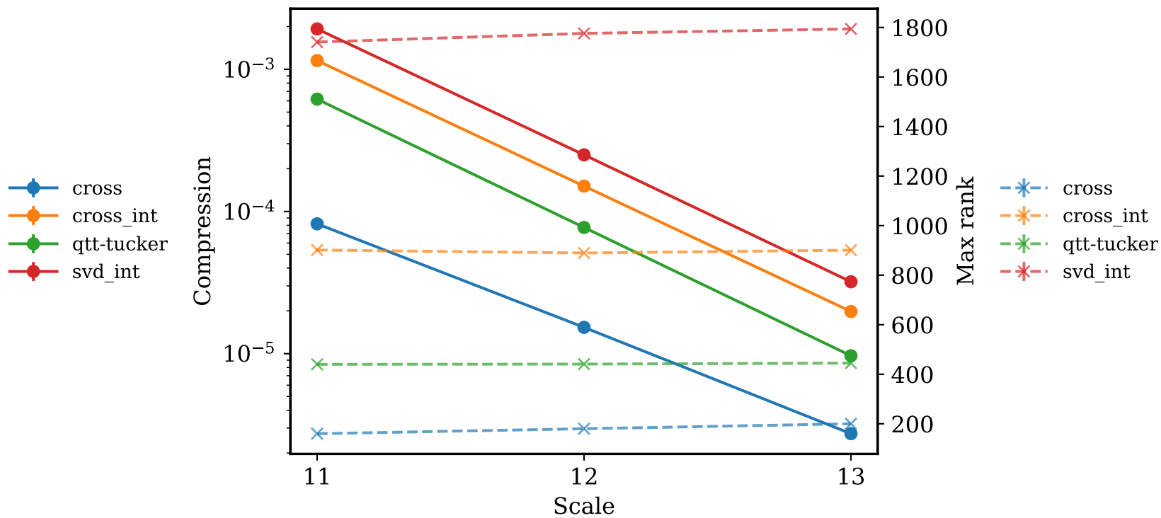
Scale vs Compression (log) & Max Rank
