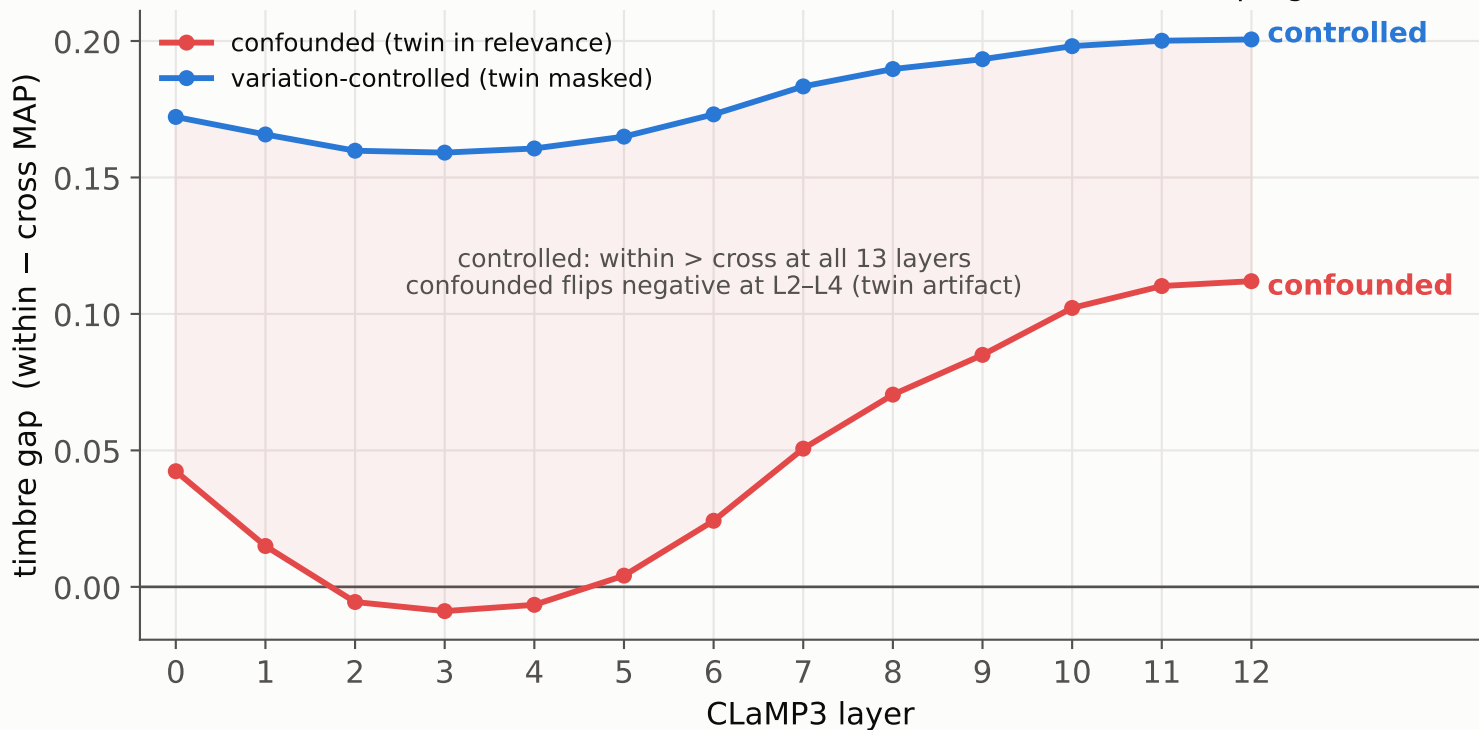
CLaMP3: the twin flips the gap negative (L2-L4) CLaMP3 · VGMIDITVar-timbre · N=102,960 · 5,040 works × 8 GM programs
