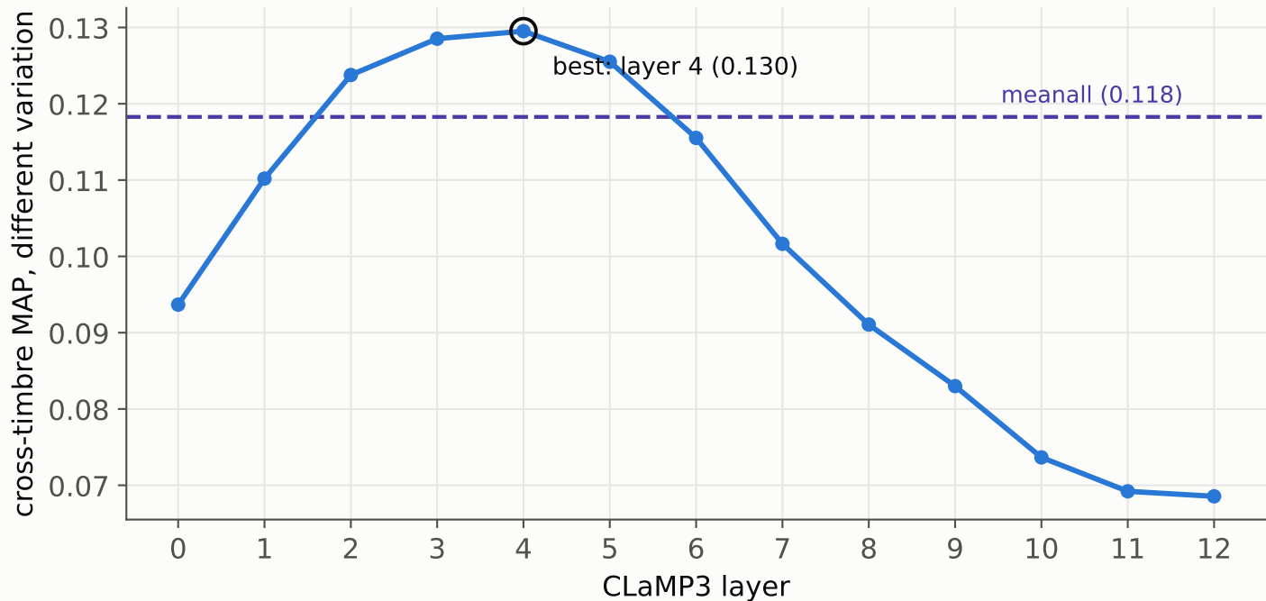
Honest cross-orchestration retrieval by depth — CLaMP3 (retrieve a different variation of the theme in a different instrument)
