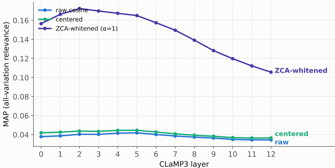
Transductive whitening lifts retrieval MAP at every layer — CLaMP3
