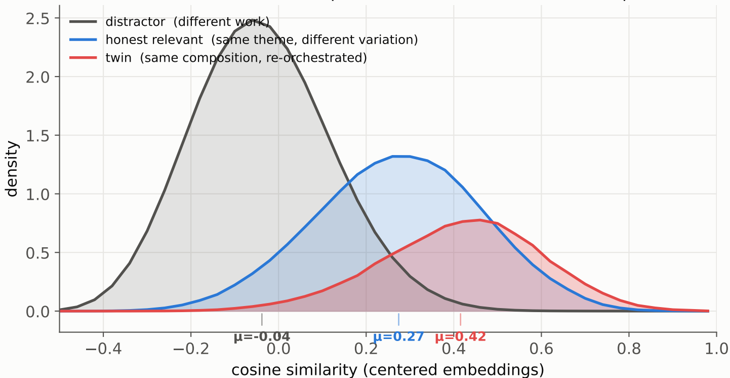
Score geometry of cross-timbre retrieval, CLaMP3 layer 4 the confound is a same-composition re-render (not a \cos \approx 1 duplicate)
