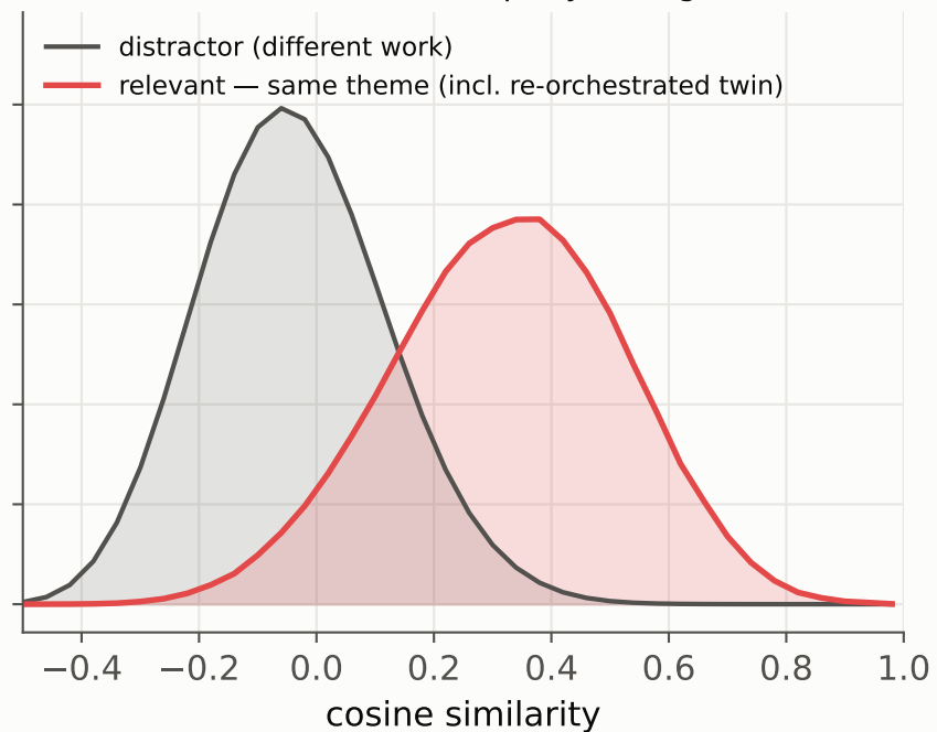
cross-timbre cells (query \neq target)
