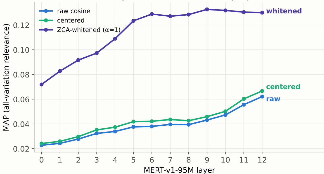
Transductive whitening lifts retrieval MAP at every layer — MERT-v1-95M
