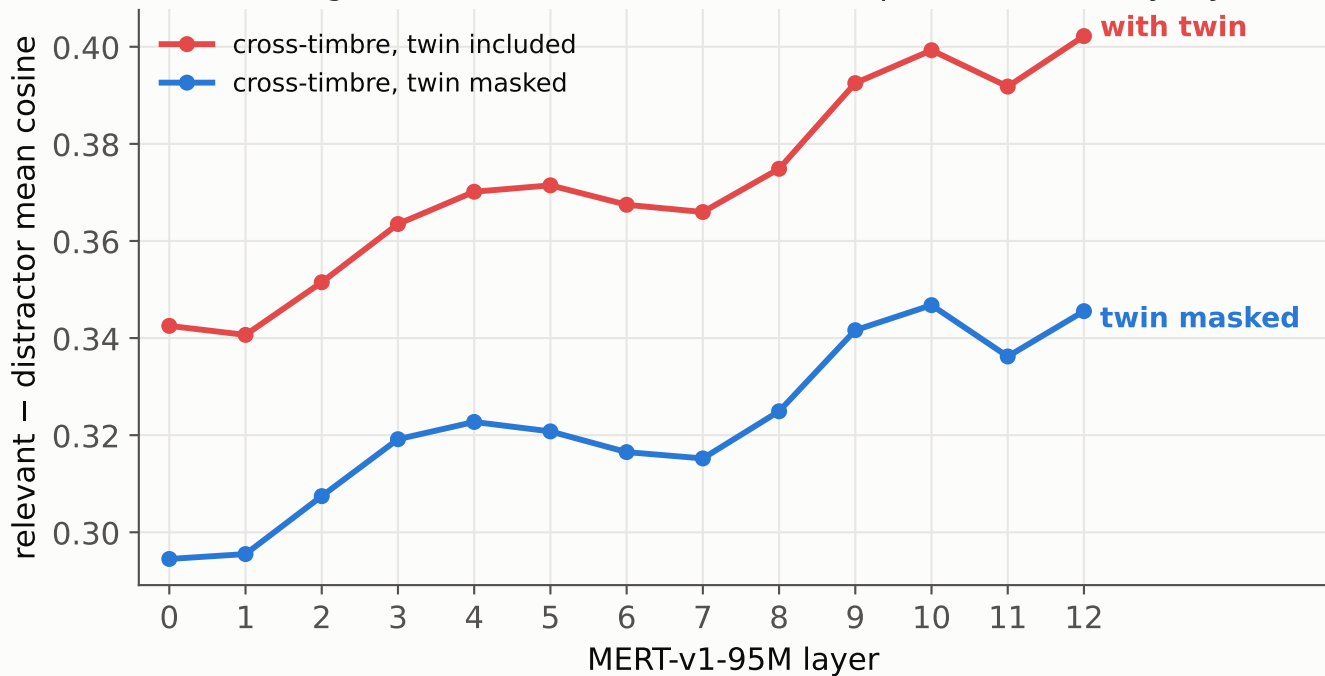
The twin's fingerprint in the raw score geometry — MERT-v1-95M (masking the twin lowers cross-timbre separation at every layer)
