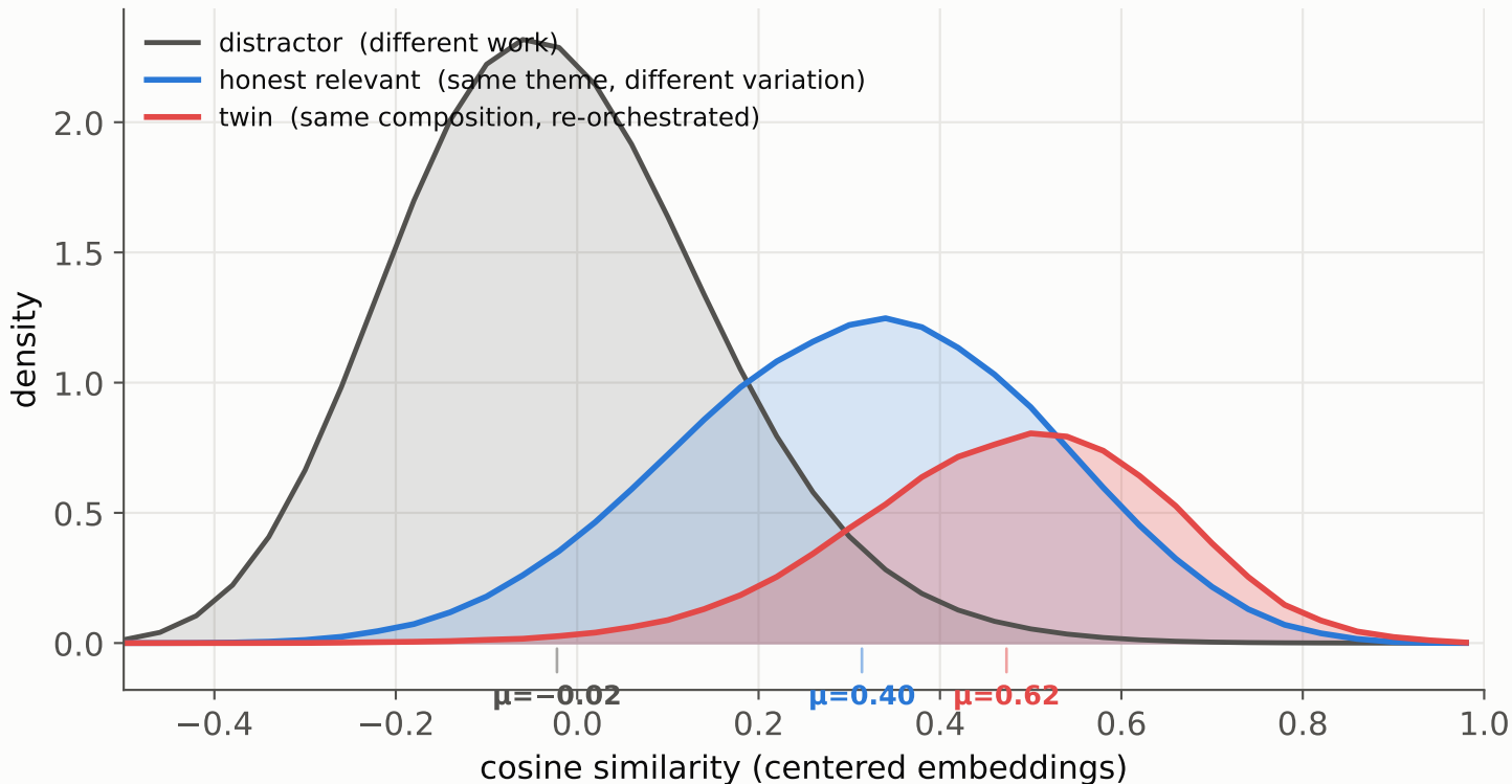
Score geometry of cross-timbre retrieval, MERT-v1-95M layer 11 the confound is a same-composition re-render (not a \cos \approx 1 duplicate)
