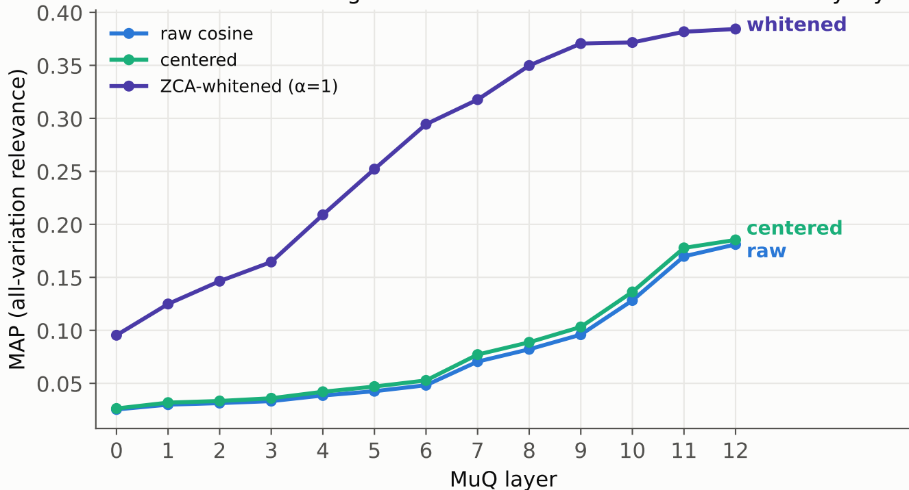
Transductive whitening more than doubles retrieval MAP at every layer
