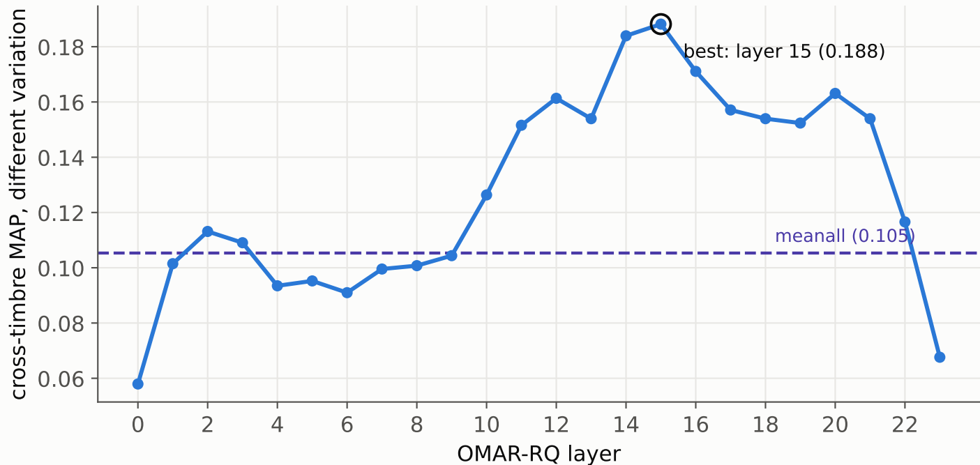
Honest cross-orchestration retrieval by depth — OMAR-RQ (retrieve a different variation of the theme in a different instrument)
