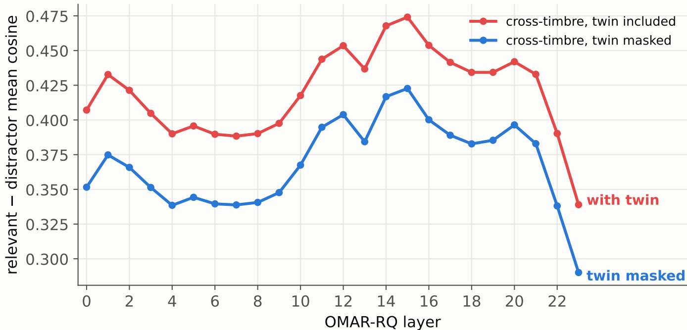
The twin's fingerprint in the raw score geometry — OMAR-RQ (masking the twin lowers cross-timbre separation at every layer)
