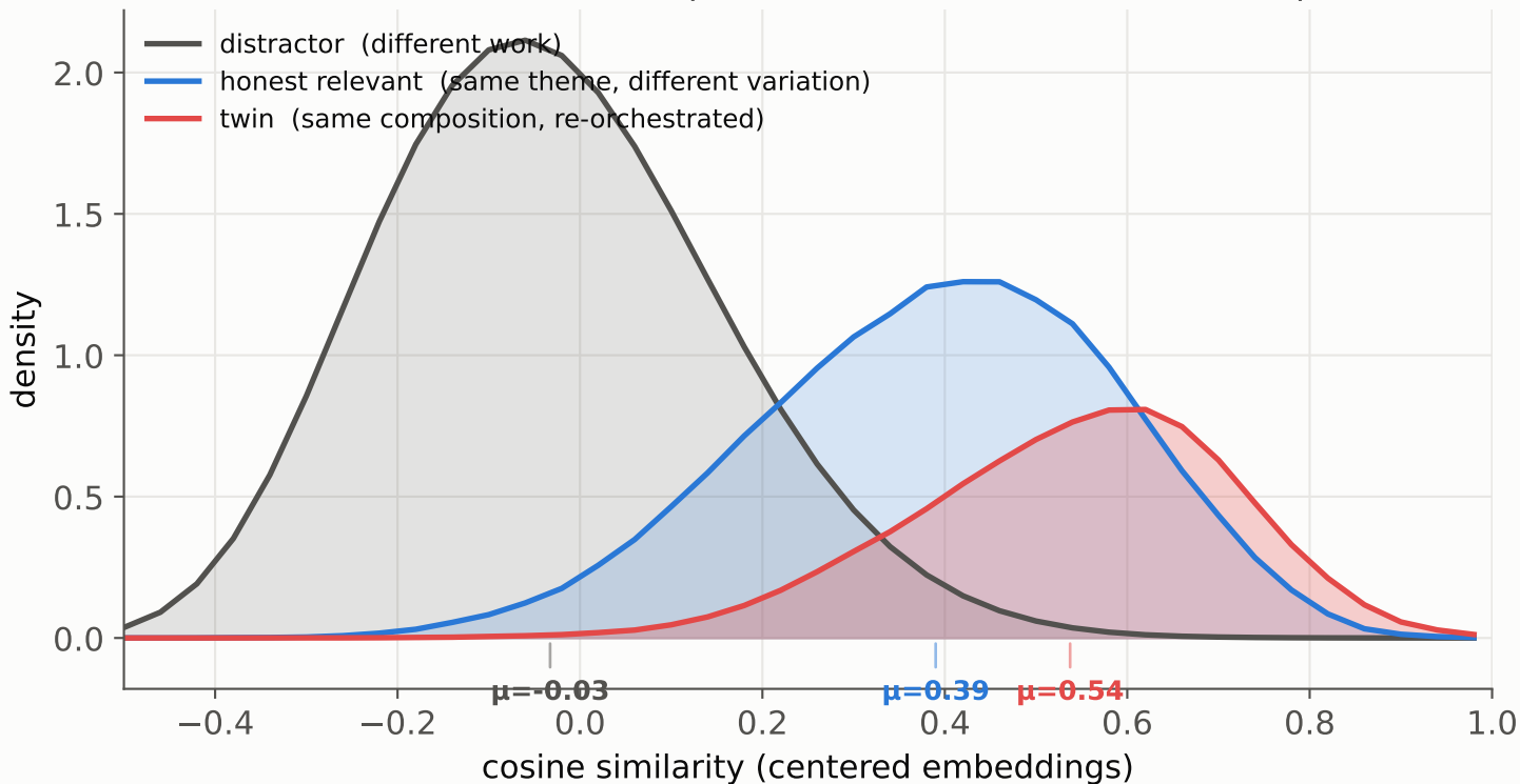
Score geometry of cross-timbre retrieval, OMAR-RQ layer 15 the confound is a same-composition re-render (not a \cos \approx 1 duplicate)
