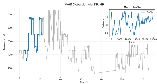
Fig. 3. Motif Detection via STUMP.
