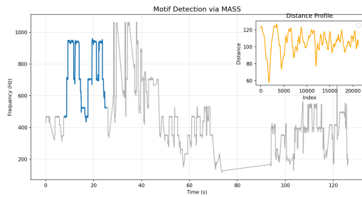
Fig. 1. Motif Detection via MASS.
