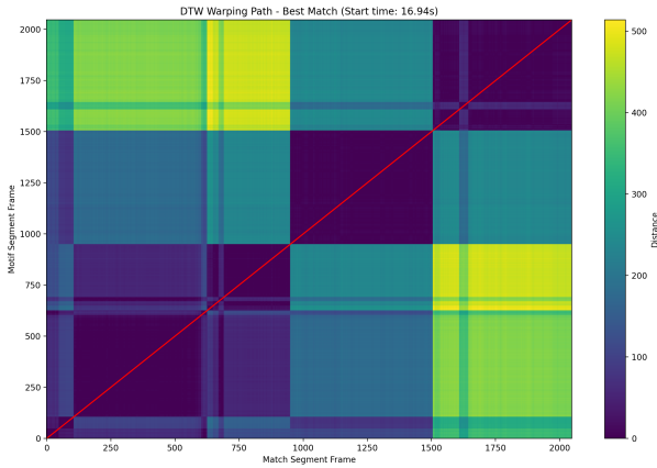
Fig. 3. DTW warping path
