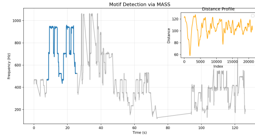
Fig. 4. Motif detection using mass algorithm.
