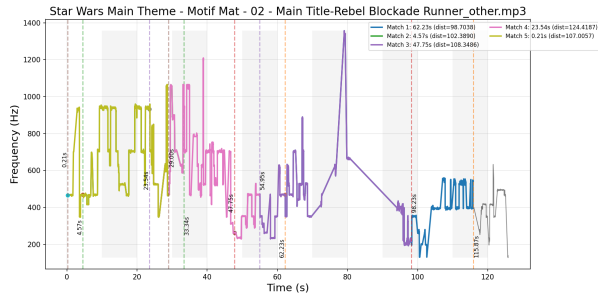
Fig. 2. Main motif detection in main theme.
