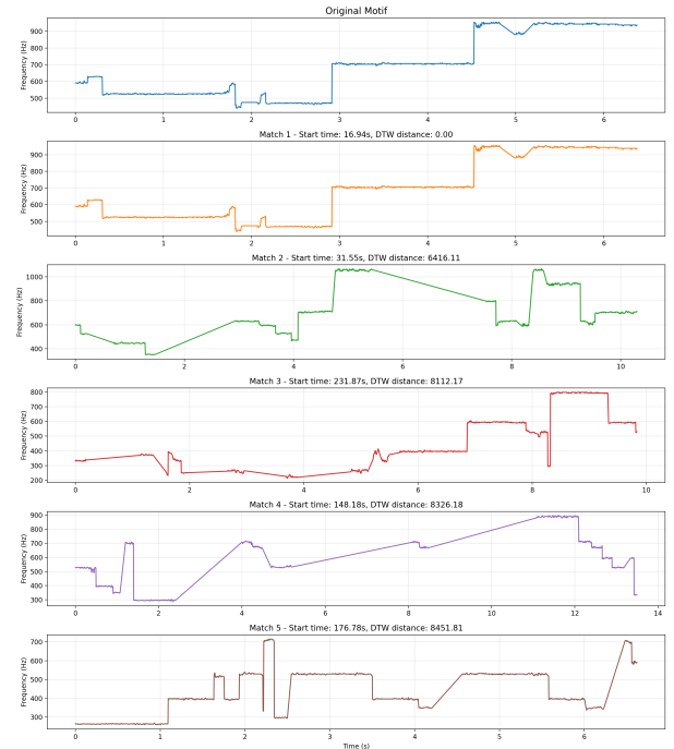
Fig. 1. DTW matches.
