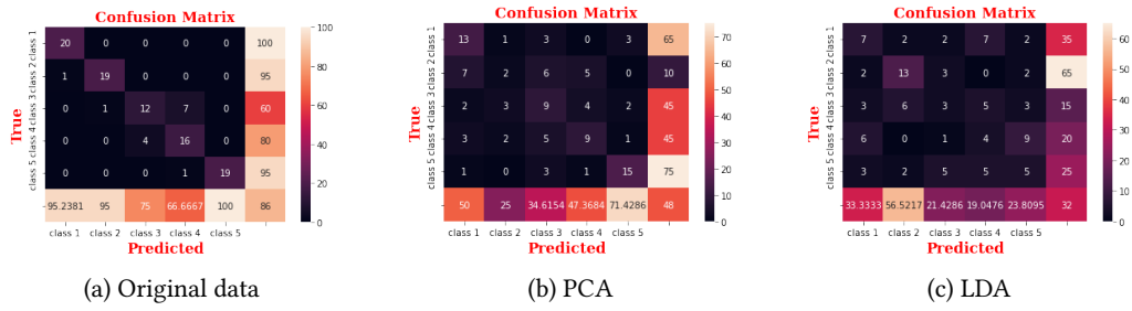
FIGURE 1.5: New dimension = 10
