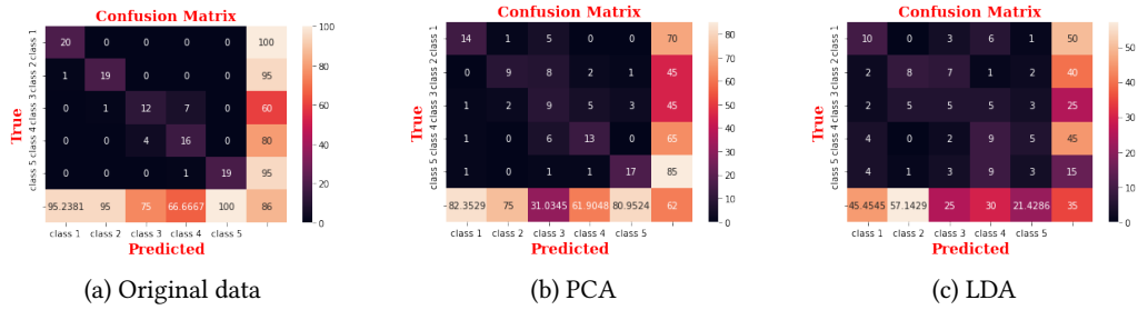
FIGURE 1.6: New dimension = 100
