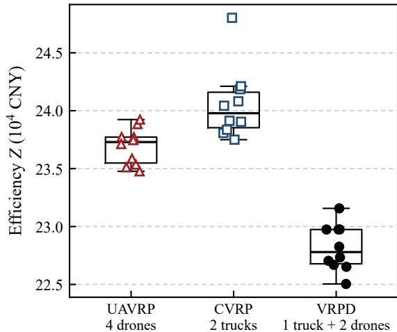
10 random instances, 20 customers each
