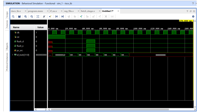
Figure 4: Behavioral simulation waveform of the RTL-based RISC-V 5-stage pipelined processor demonstrating instruction fetch, decode activity, and pipeline flushing during hazard resolution.
