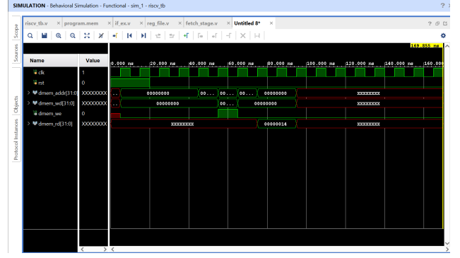
Figure 5: Behavioral simulation waveform of the RTL-based RISC-V pipelined processor illustrating Data Memory (D-Mem) read and write operations during execution. The waveform shows the initialization phase with undefined memory states, followed by a successful memory write operation during a Store instruction when dmem_we is asserted. A subsequent memory read operation retrieves the hexadecimal value 00000014 from memory, confirming correct Load instruction functionality. Toward the end of the simulation interval, undefined values appear on the address and data buses, indicating access to uninitialized or unmapped memory regions after completion of the programmed instruction sequence.
