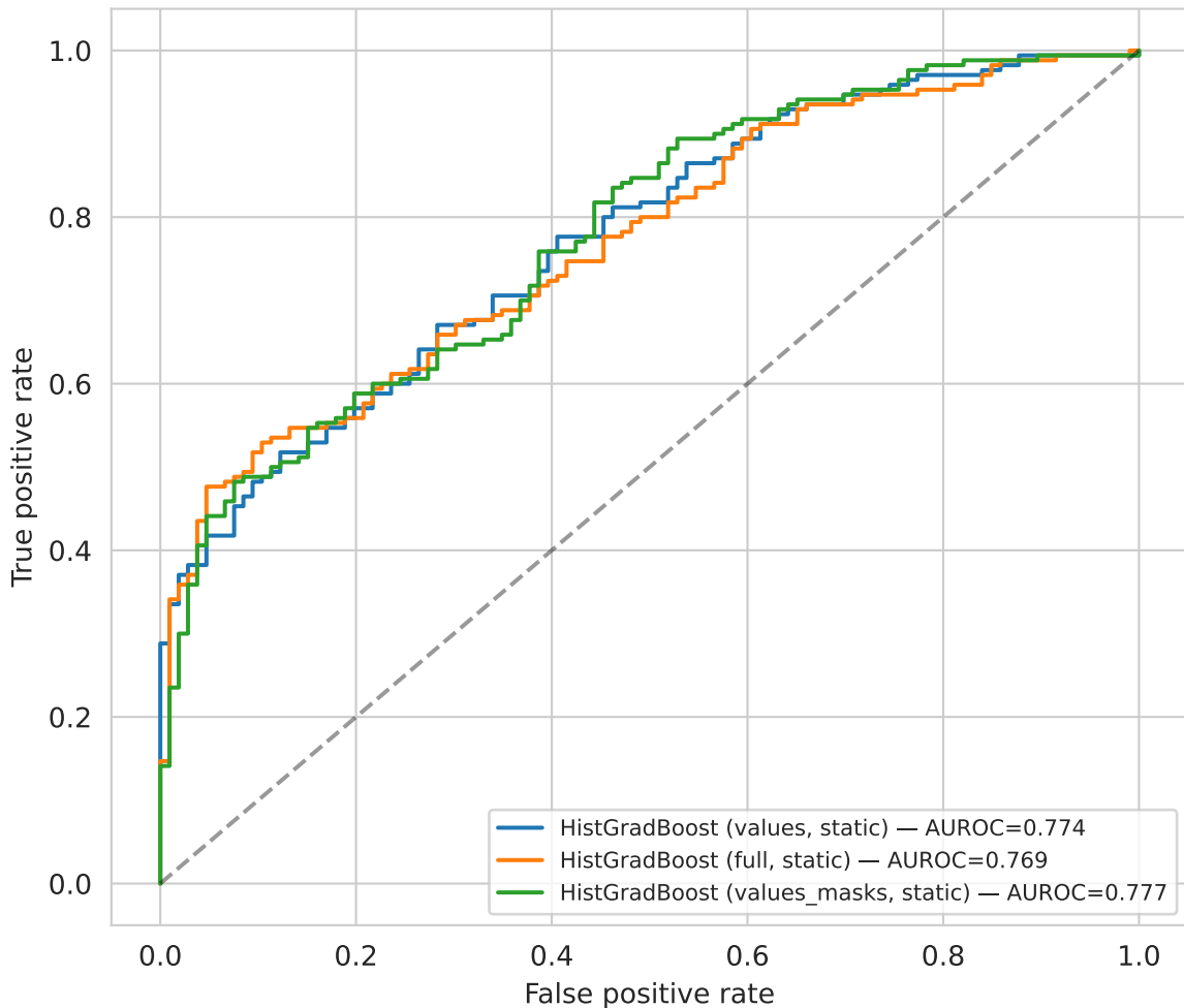
Top models — ROC at 18h
