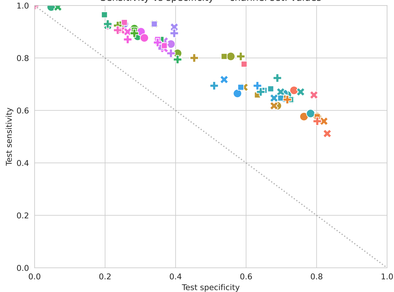
Sensitivity vs specificity — channel set: values
