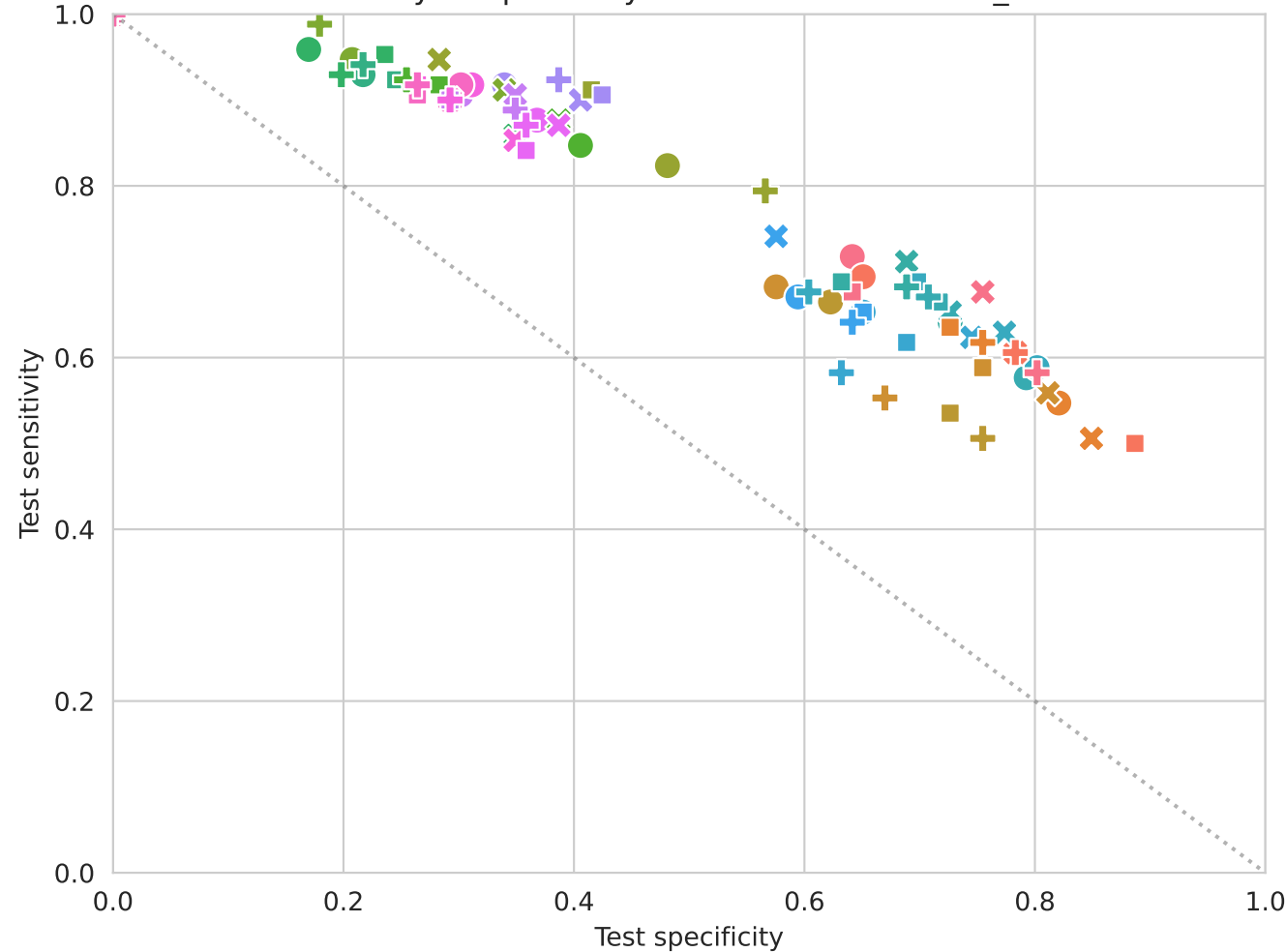
Sensitivity vs specificity — channel set: values_masks
