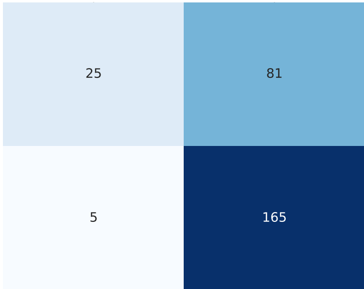
Test confusion matrix @ thr=0.184
