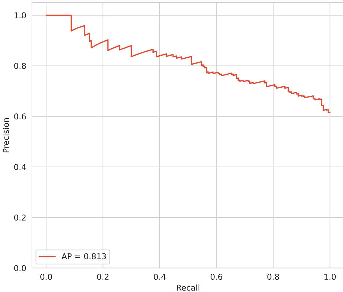
Test Precision-Recall
