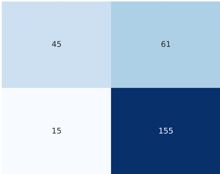
Test confusion matrix @ thr=0.327
