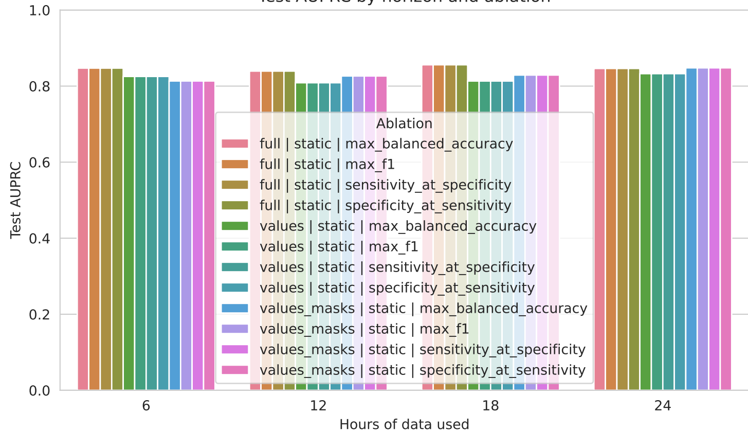
Test AUPRC by horizon and ablation
