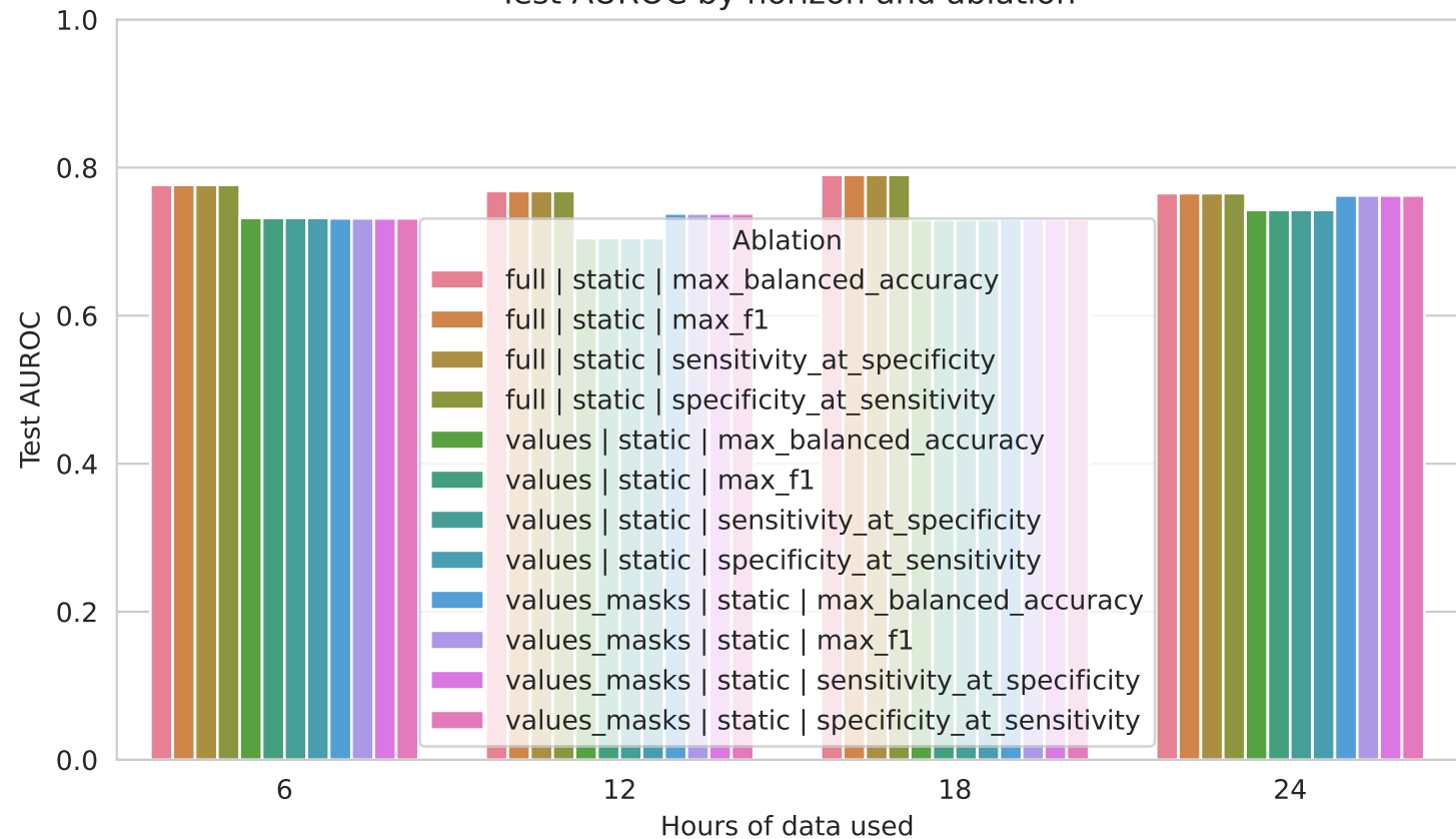
Test AUROC by horizon and ablation
