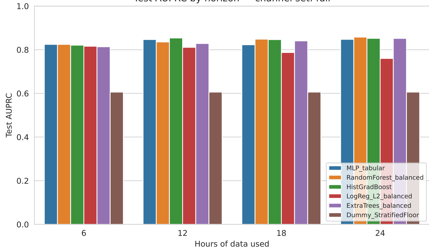
Test AUPRC by horizon — channel set: full
