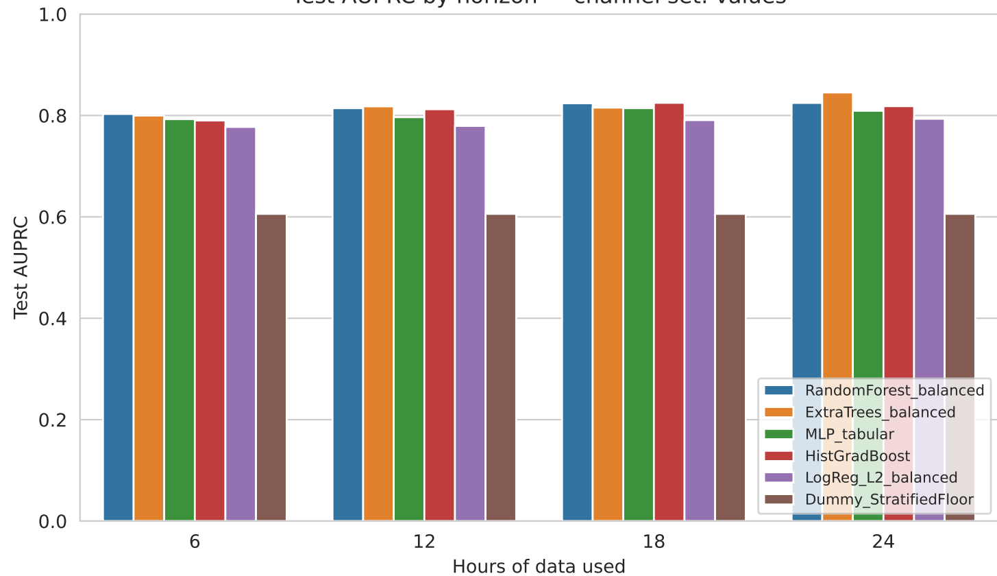
Test AUPRC by horizon — channel set: values
