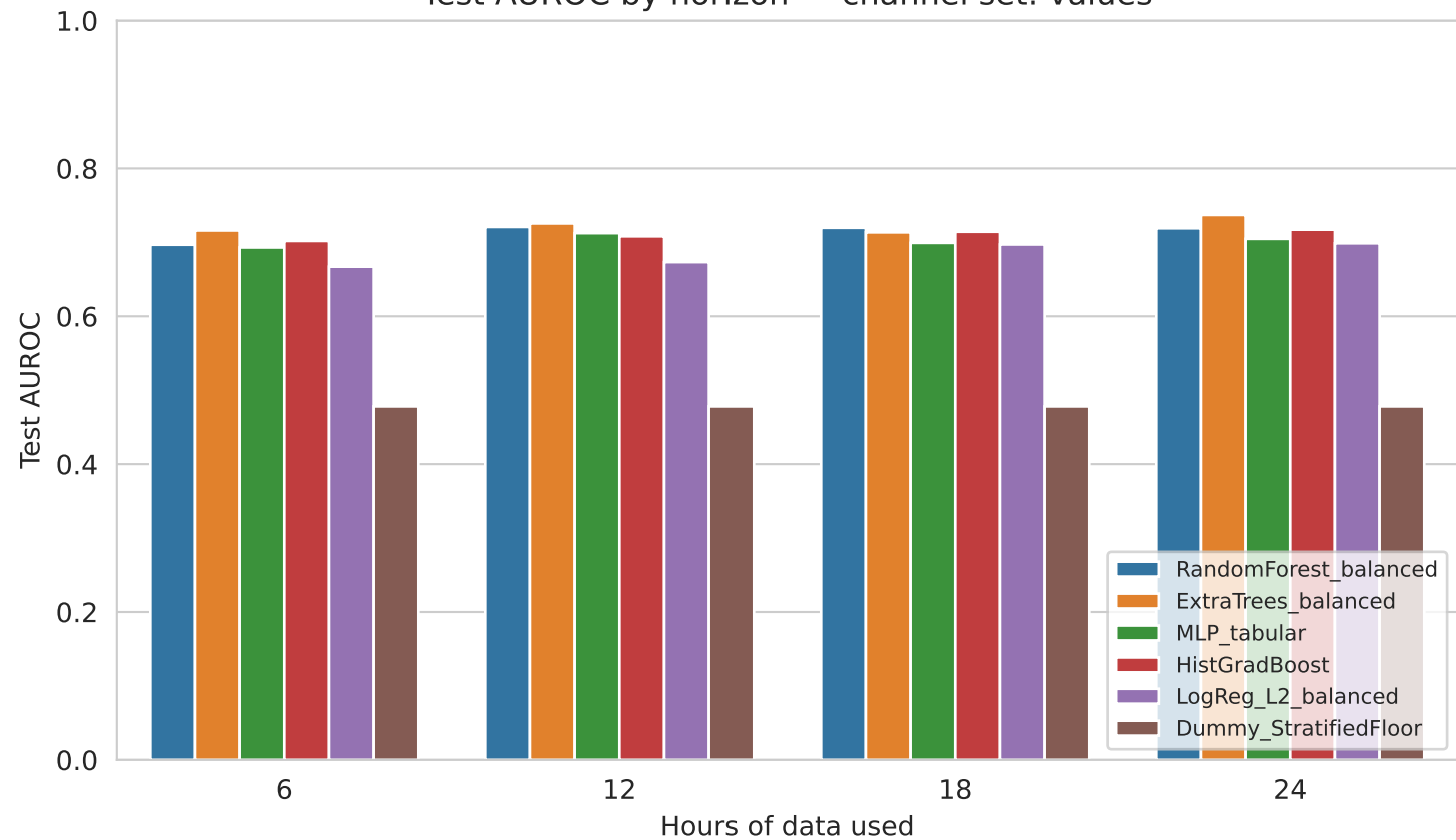
Test AUROC by horizon — channel set: values
