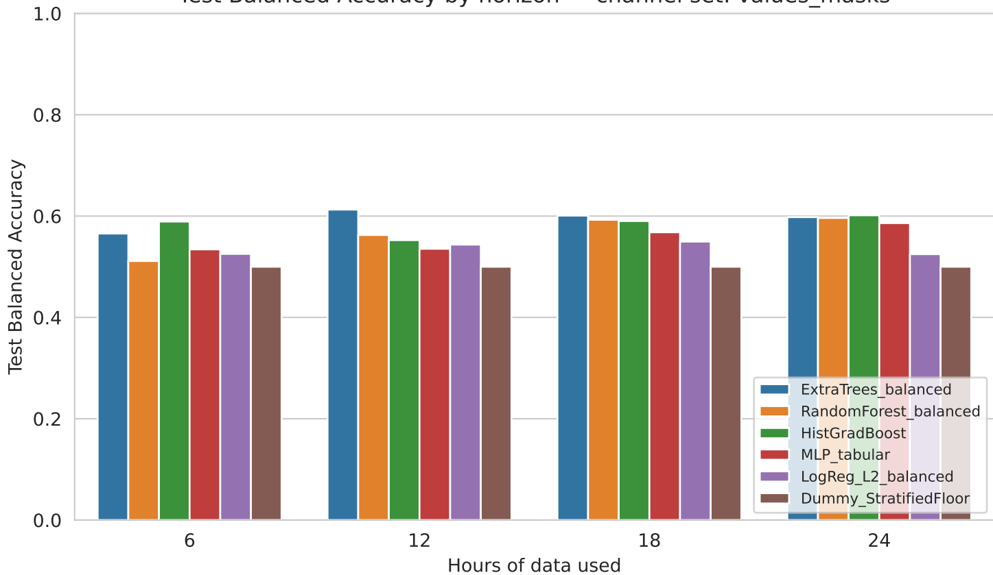
Test Balanced Accuracy by horizon — channel set: values_masks
