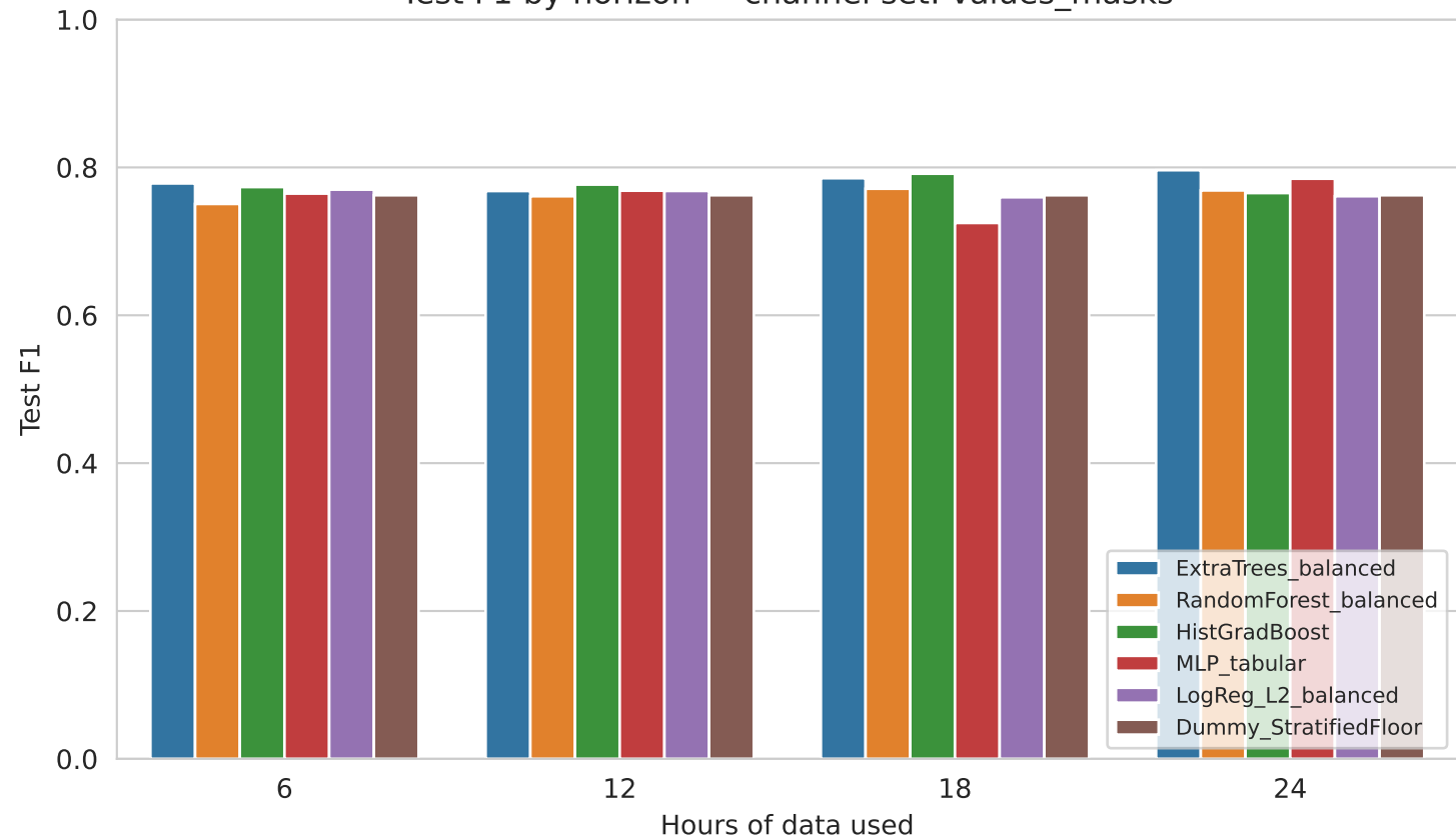
Test F1 by horizon — channel set: values_masks
