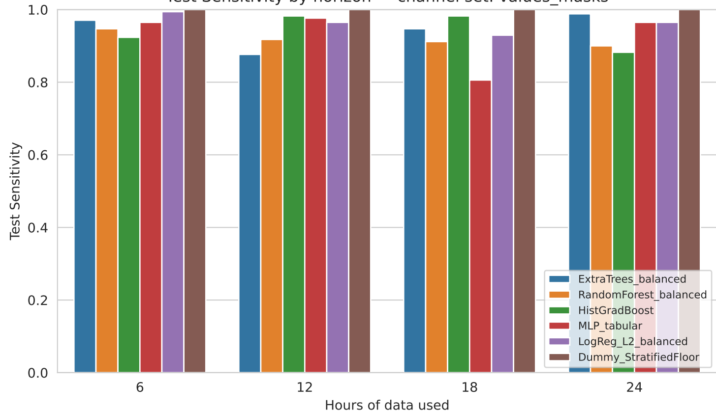
Test Sensitivity by horizon — channel set: values_masks
