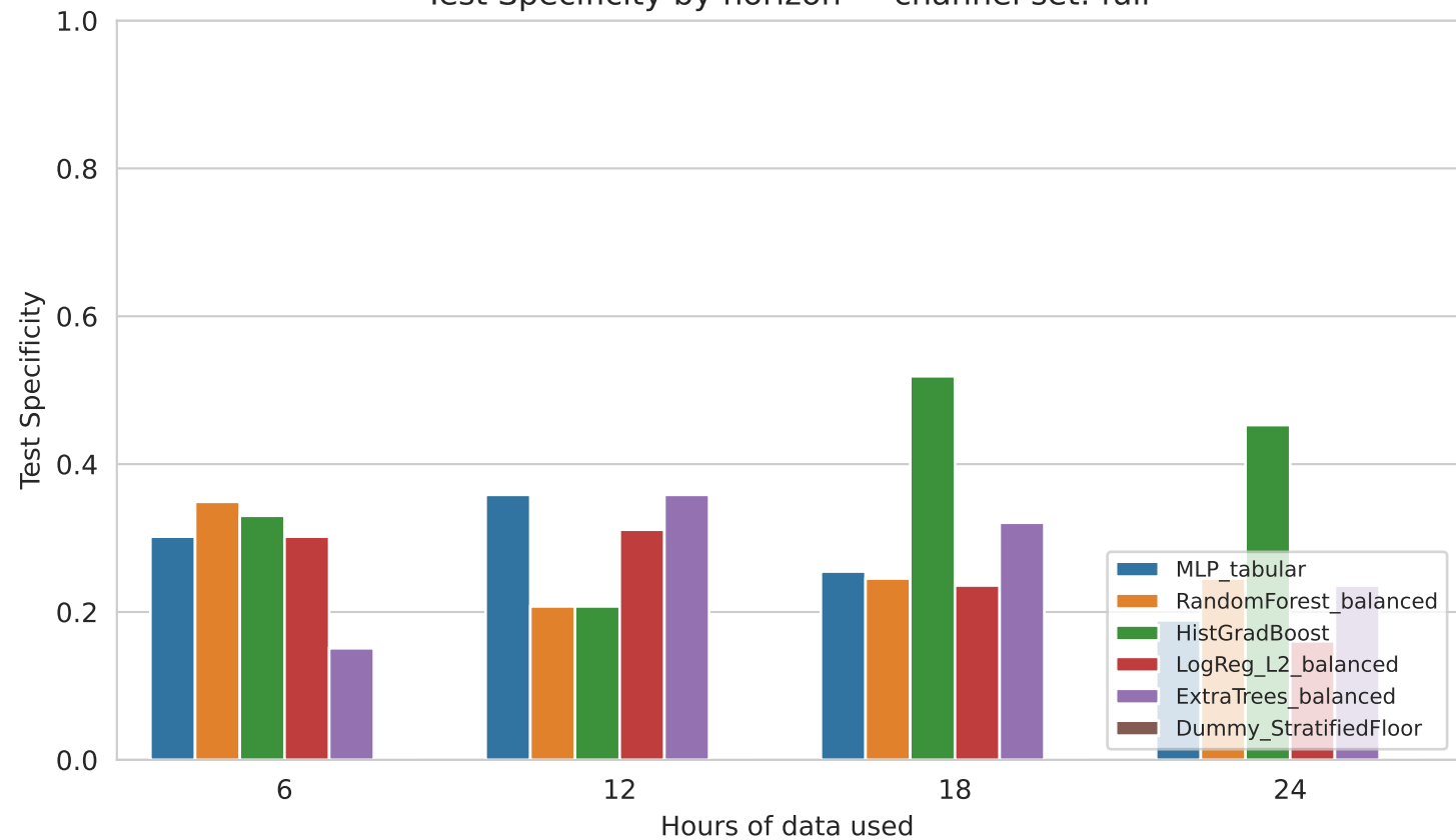
Test Specificity by horizon — channel set: full
