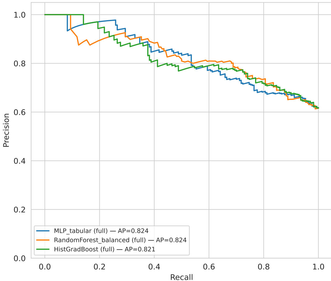
Top models — PR at 6h
