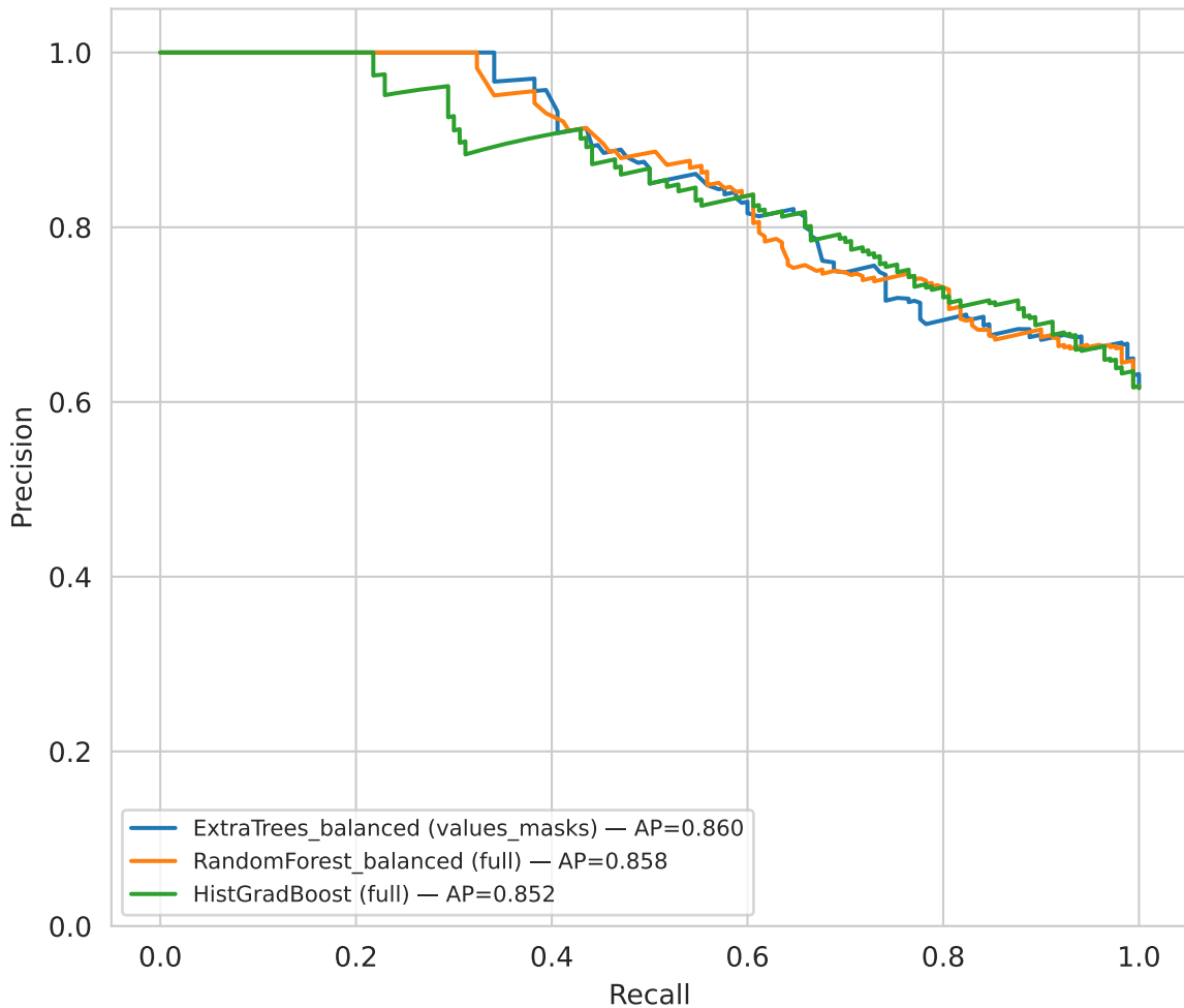
Top models — PR at 24h
