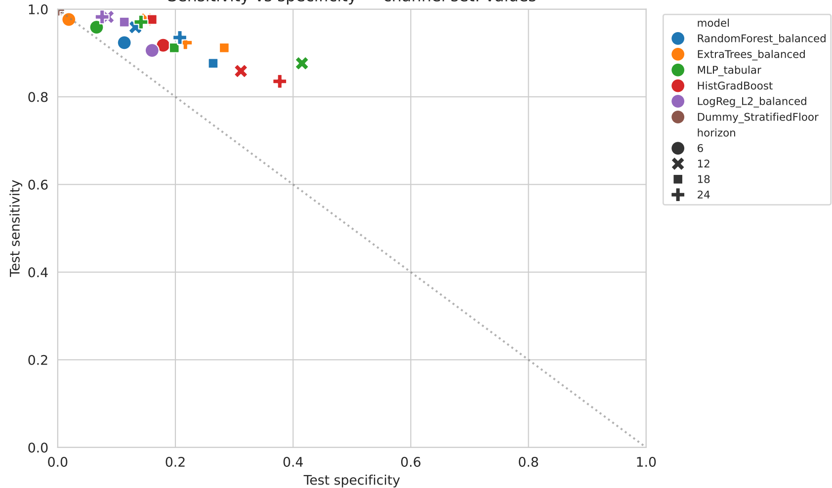
Sensitivity vs specificity — channel set: values
