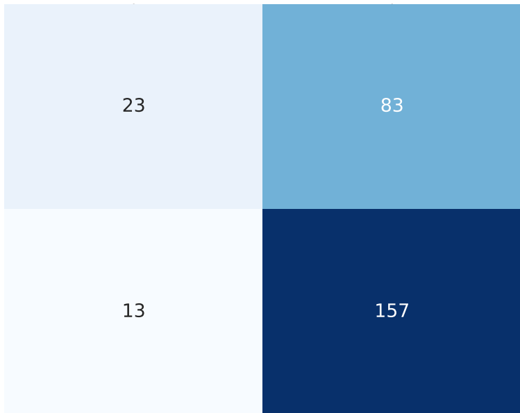
Test confusion matrix @ thr=0.190
