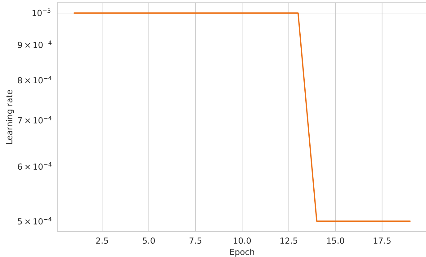
Learning rate schedule
