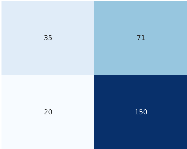
Test confusion matrix @ thr=0.336
