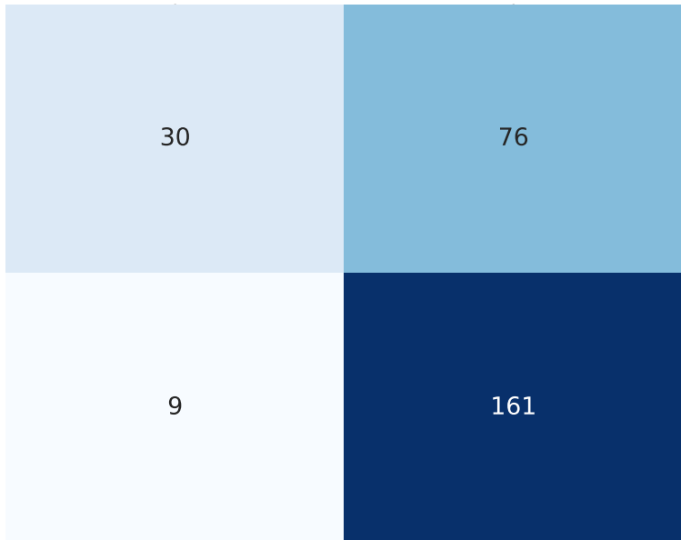
Test confusion matrix @ thr=0.224
