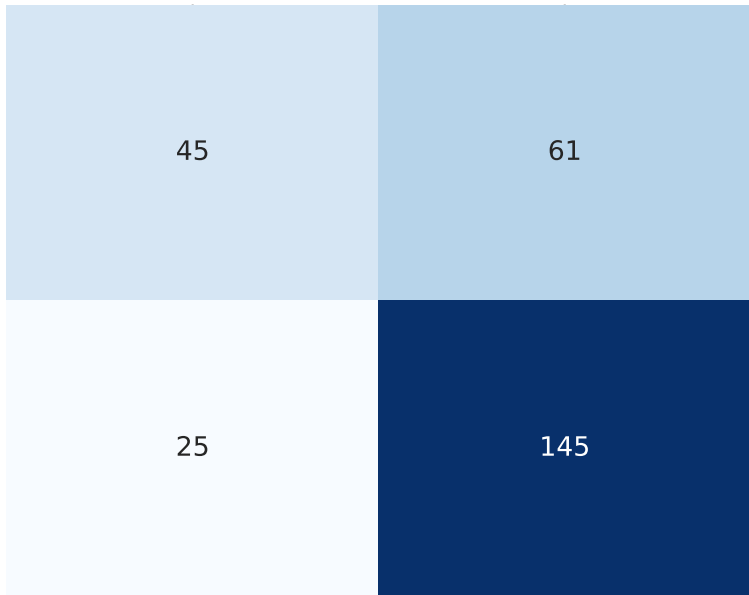
Test confusion matrix @ thr=0.363
